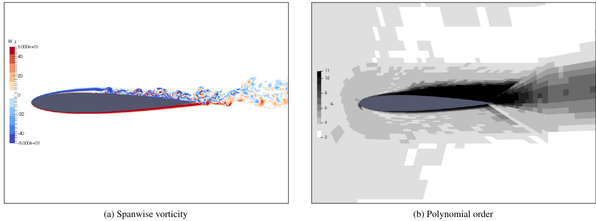
Fig. 5. Polynomial order and vorticity distributions obtained with simulation using adaptive polynomial order for the flow around a NACA 0012 profile with Re = 50,000 and \alpha = 6^\circ .
