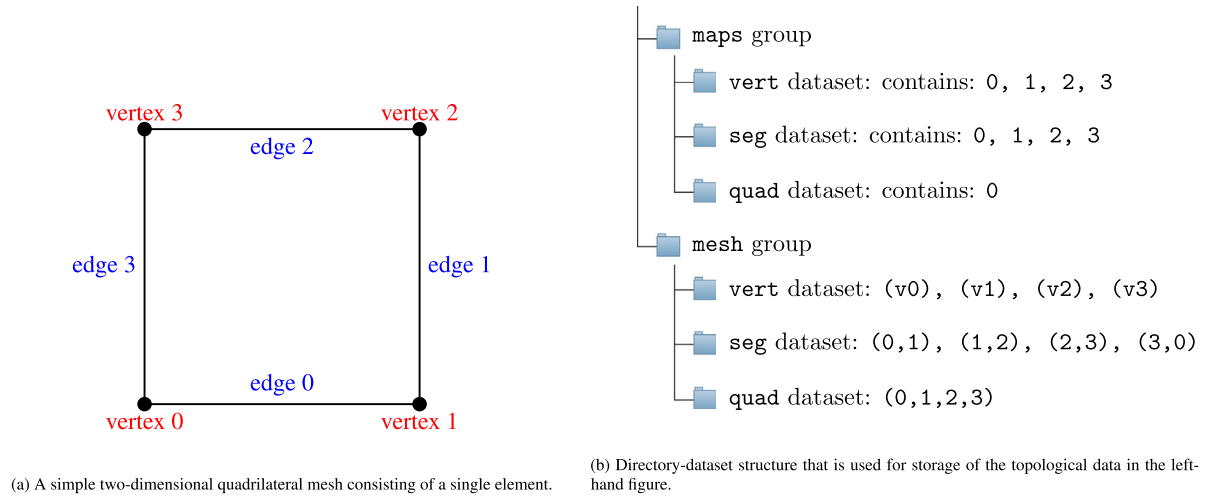
Fig. 2. An example of a single quadrilateral element grid. In (a), we show the topological decomposition of the element into its 4 edges and vertices. Figure (b) shows a schematic of the filesystem-type structure implemented in HDF5 that is used for storage of this topological information.
