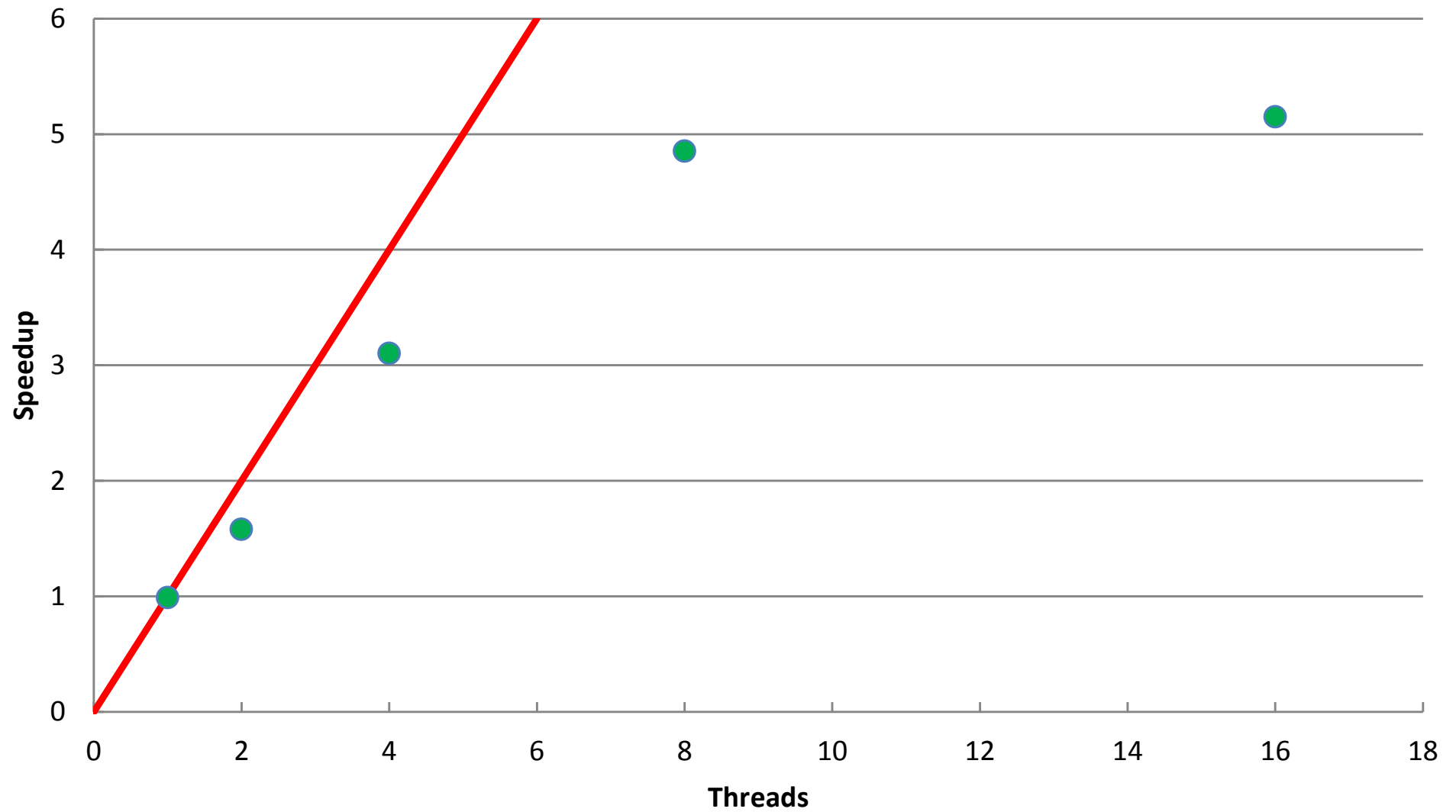
SPades speedup vs. Threads
